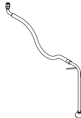
SUCTION HOSE ASSEMBLY 0115-010236 20 L (20 MESH) 0115-010381 200 L (30 MESH) 0115-010106 Tripod Inlet Tube (16 MESH) Service Bulletin 77-2923
