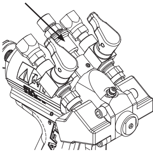
Air Switch
